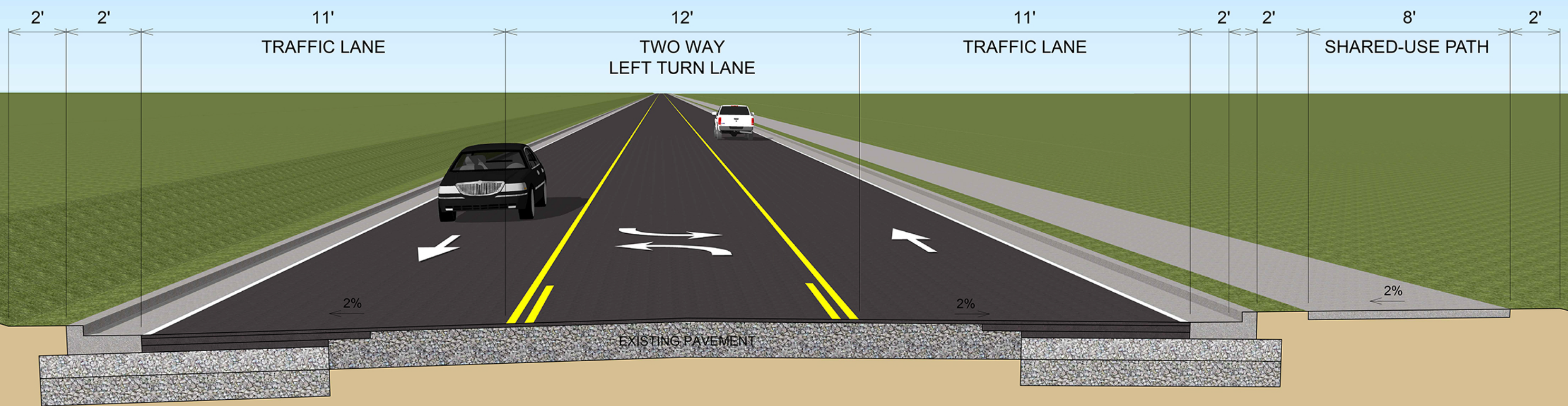
TYPICAL SECTION
